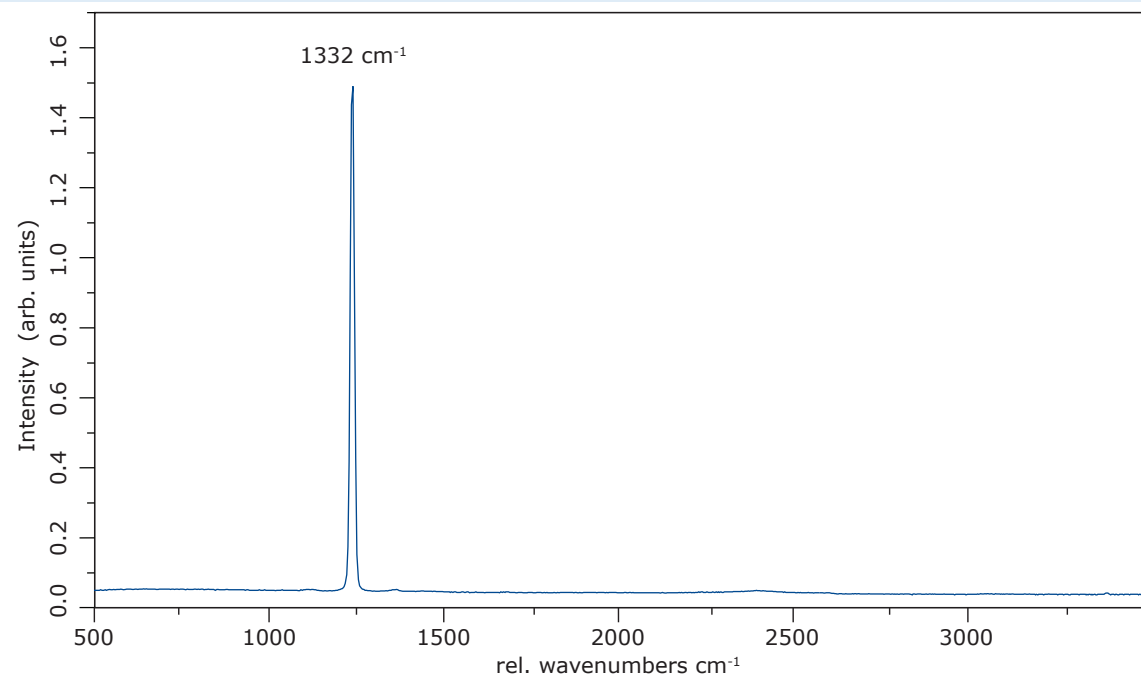
First order Raman spectrum of a type IIa diamond anvil with Raman low fluorescence selection
