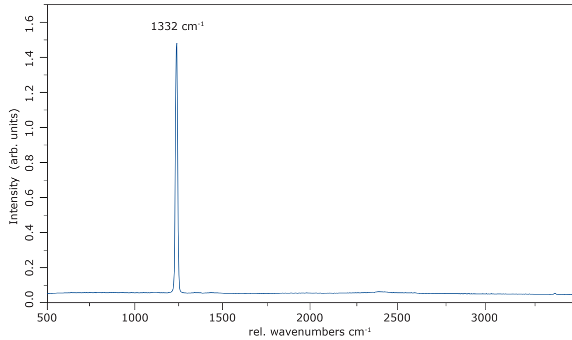
First order Raman spectrum of a type IIa diamond anvil without Raman selection
