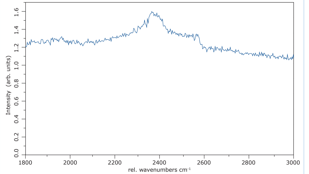
Second order Raman spectrum of a type IIa diamond anvil without Raman selection
