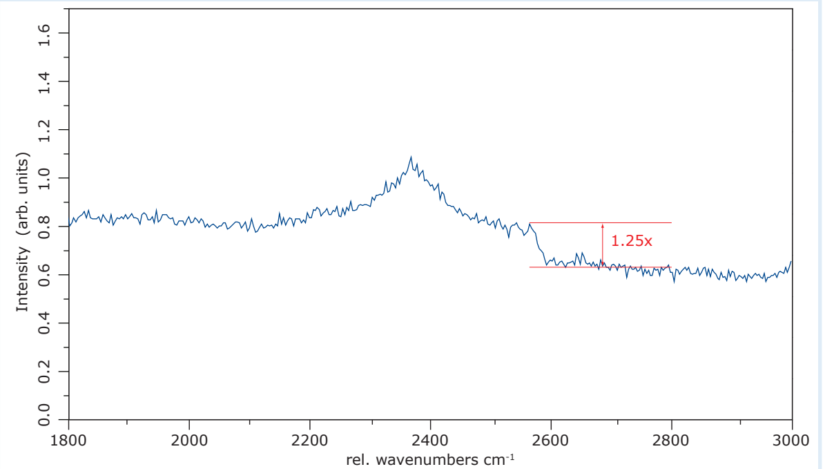
Second order Raman spectrum of a type IIa diamond anvil with Raman low fluorescence selection
