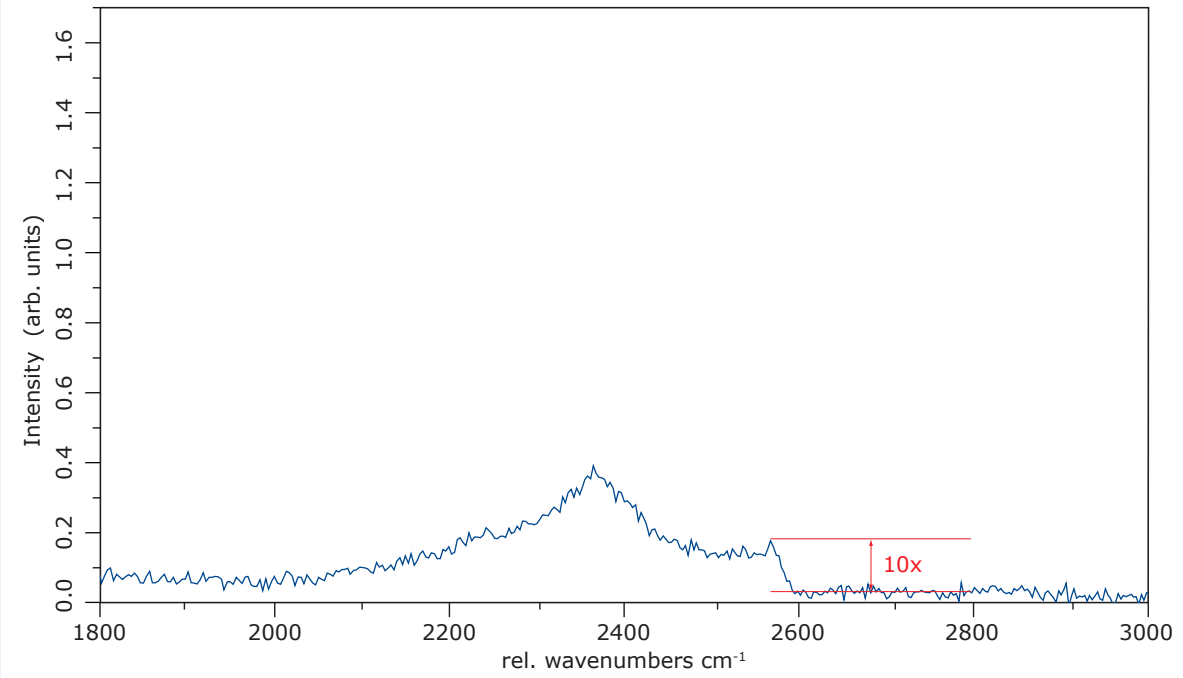
Second order Raman spectrum of a synthetic type IIas diamond anvil with Raman ultra low fluorescence selection
