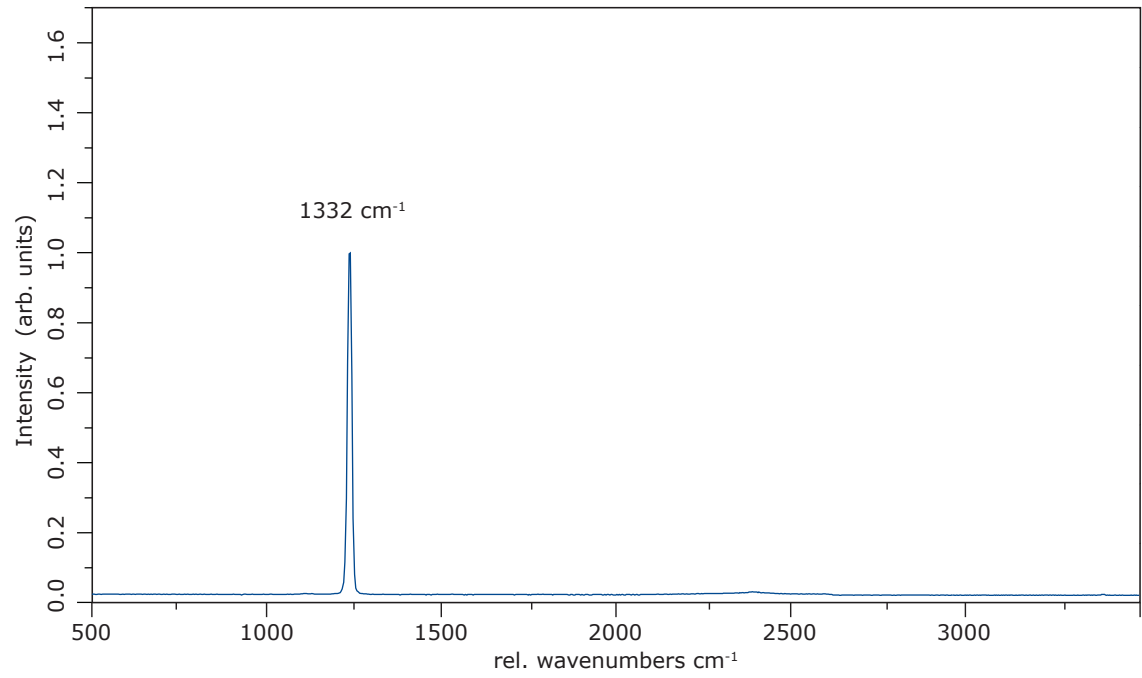
First order Raman spectrum of a synthetic type IIas diamond anvil with Raman ultra low fluorescence selection
