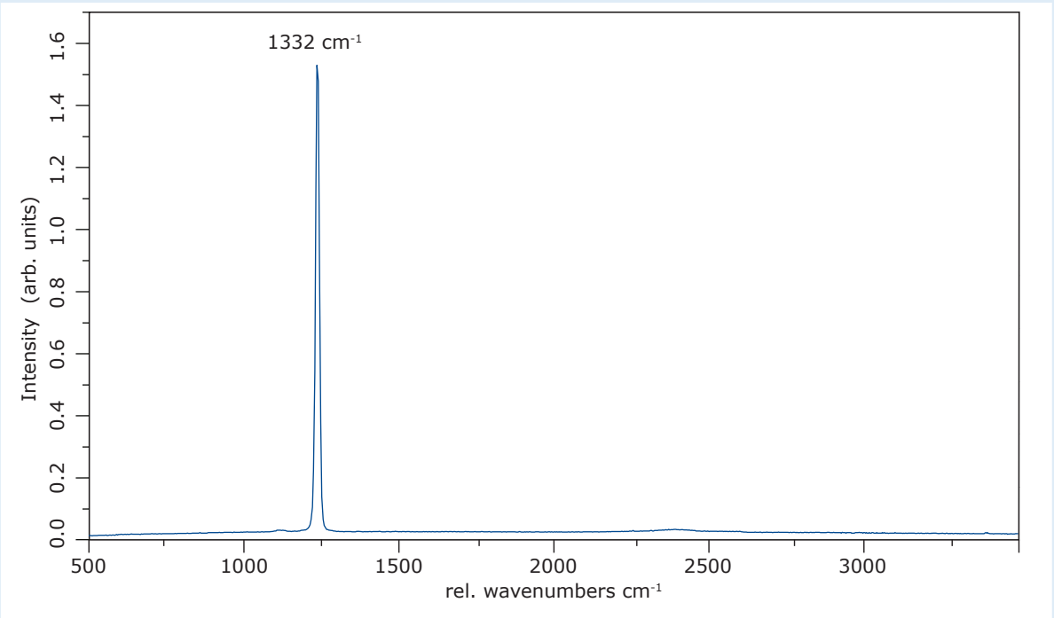
First order Raman spectrum of a type Ia diamond anvil without Raman selection
