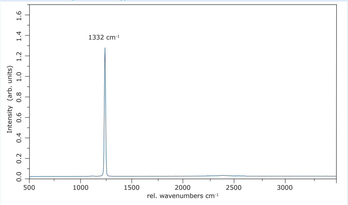
First order Raman spectrum of a type Ia diamond anvil with Raman low fluorescence selection
