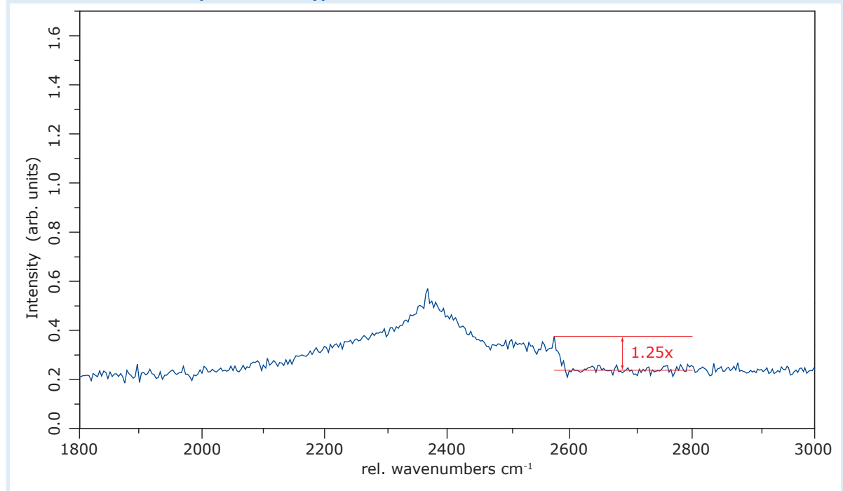
Second order Raman spectrum of a type Ia diamond anvil with Raman low fluorescence selection
