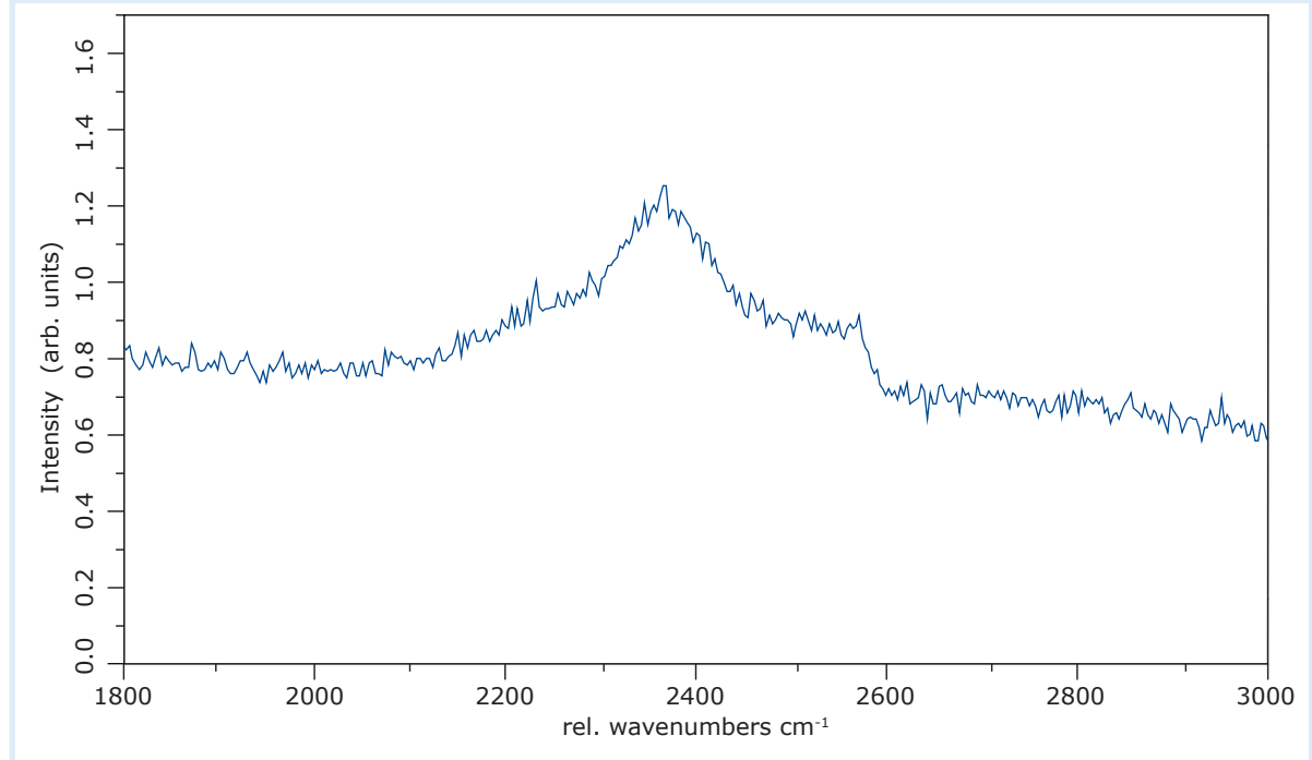
Second order Raman spectrum of a type Ia diamond anvil without Raman selection
