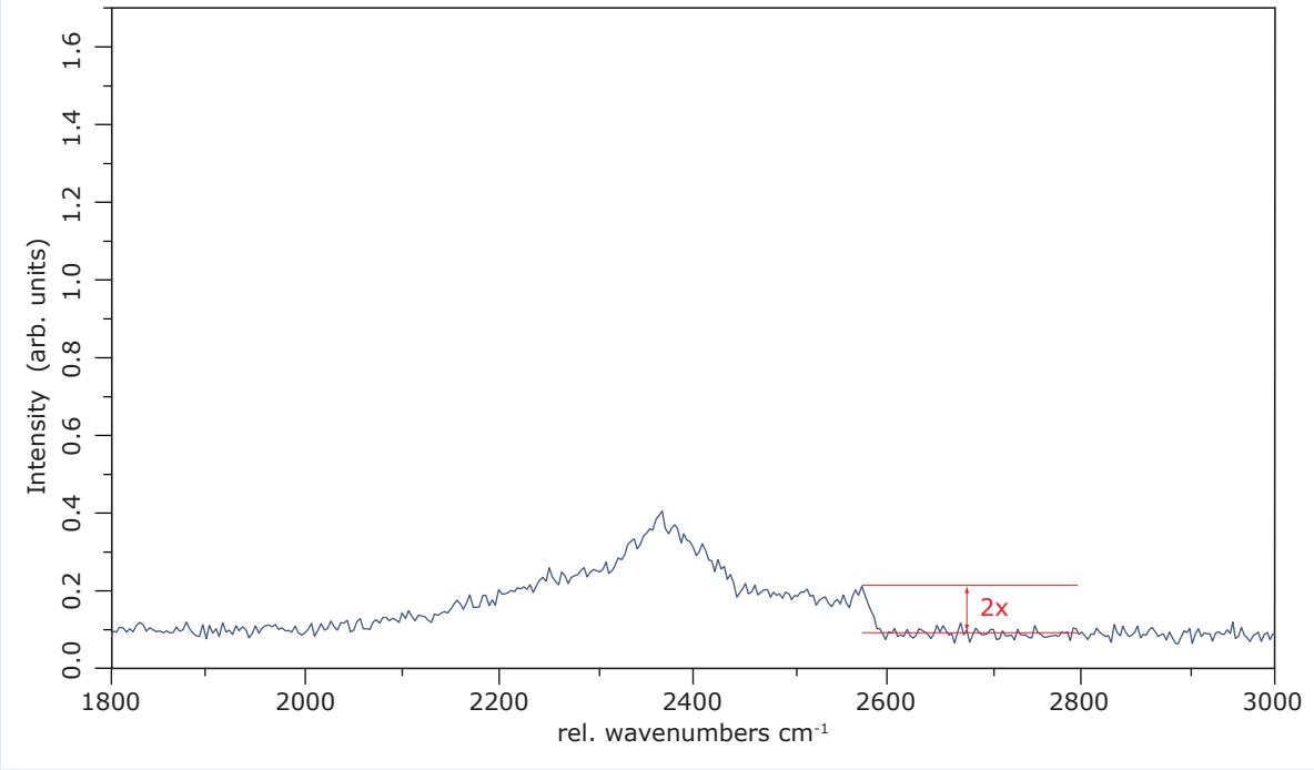
Second order Raman spectrum of a type Ia diamond anvil with Raman ultra low fluorescence selection
